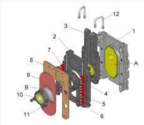
Slide gate mechanism for BOF
